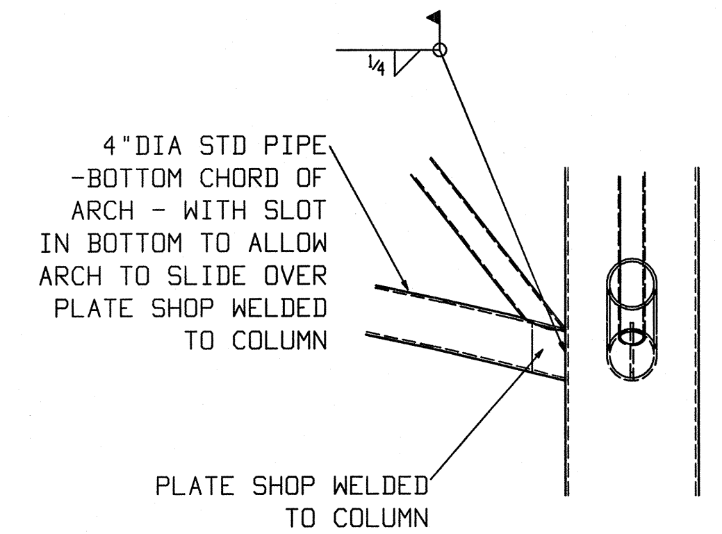
DETAIL B
