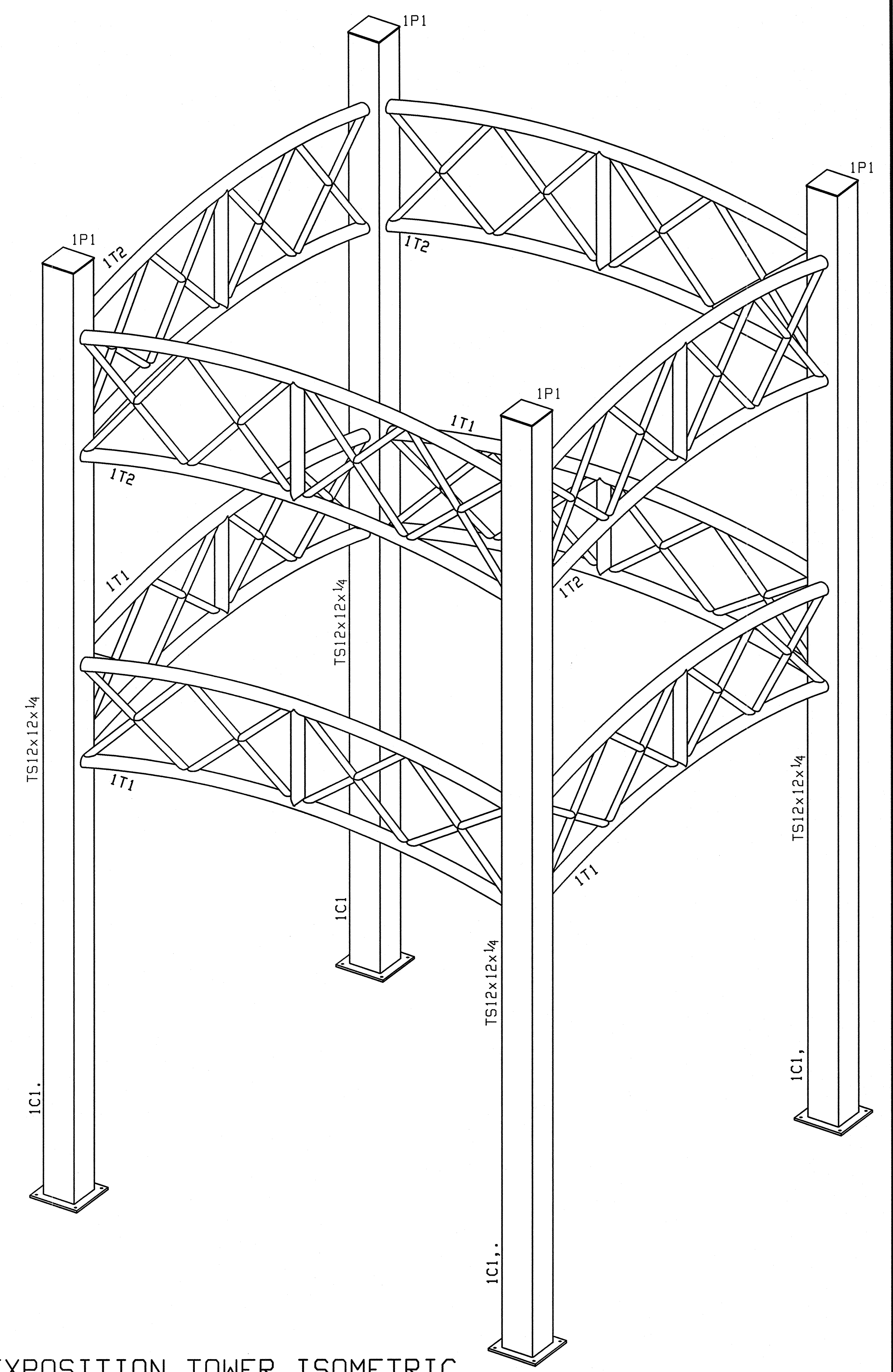
EXPOSITION TOWER ISOMETRIC
